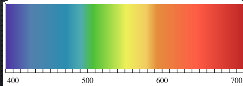
Visible light spectrum
